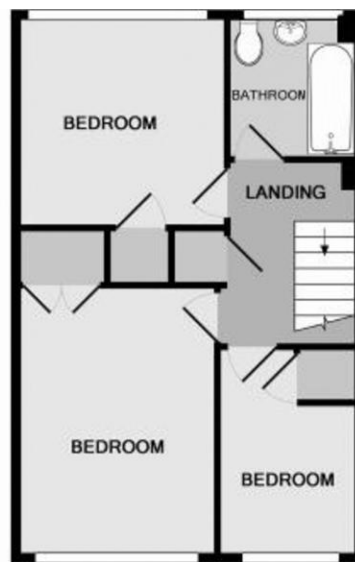
1ST FLOOR APPROX. FLOOR AREA 410 SQ.FT. (38.1 SQ.M.)
